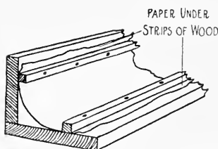
FIG. 528. WOOD FILLET PLACED.
